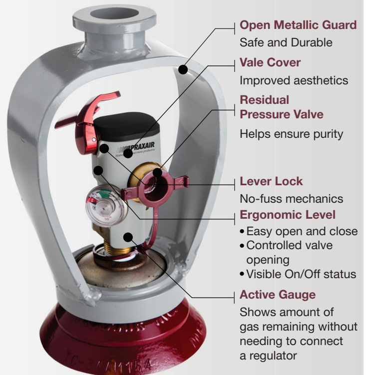
From View Valve Open
